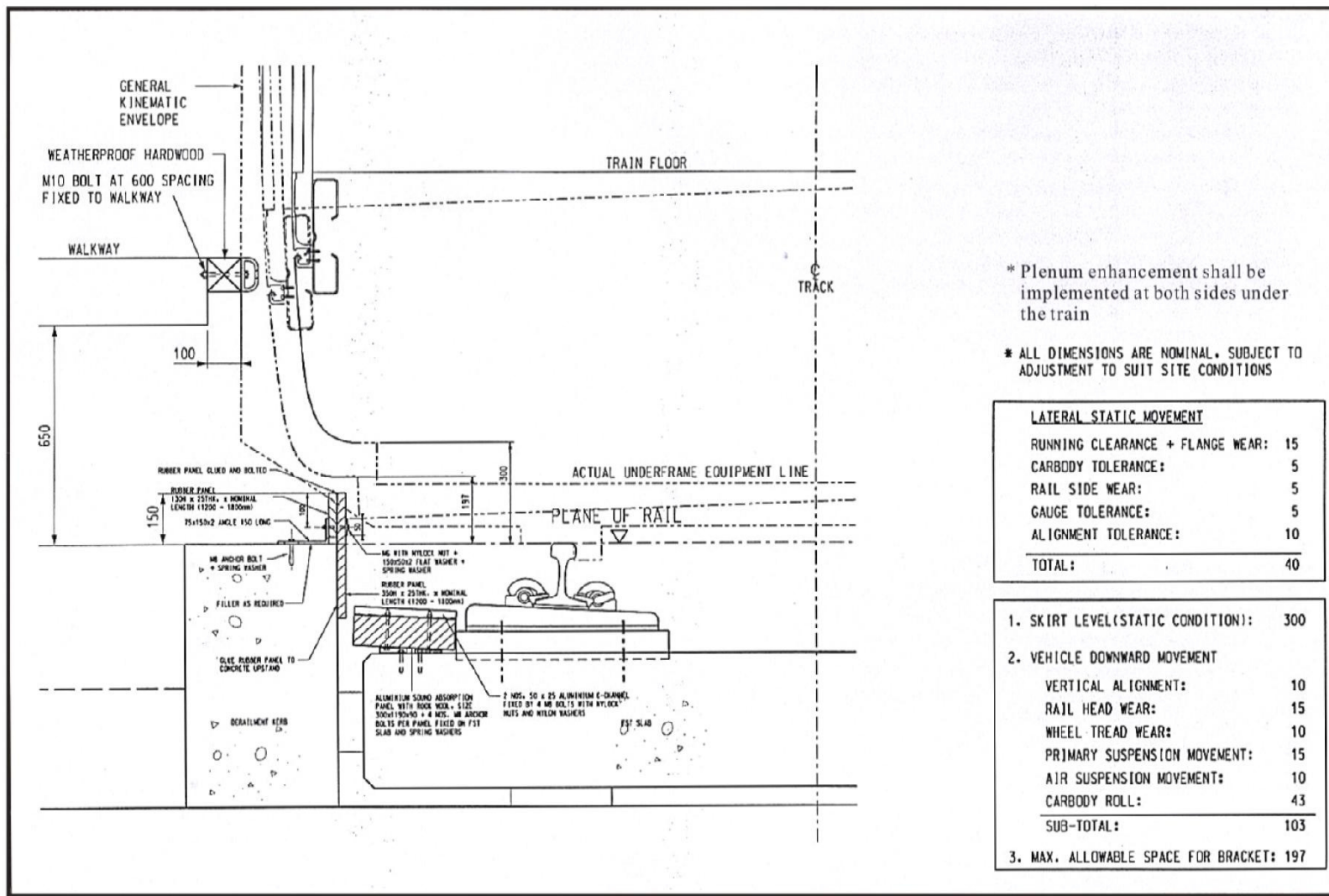
Figure 8 – Additional Noise Mitigation Measure on the Viaducts
